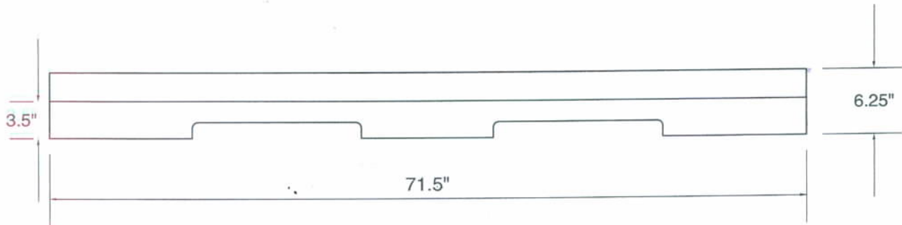
SIDE VIEW
